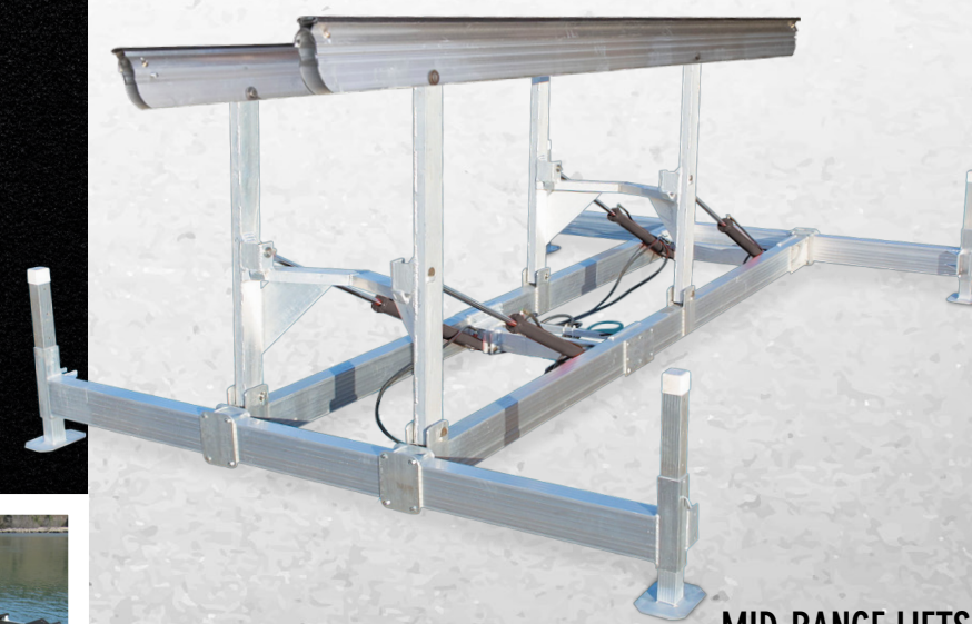
MID-RANGE LIFTS 8100 and 10,100 lb Lifts (Four hydraulic cylinders)
